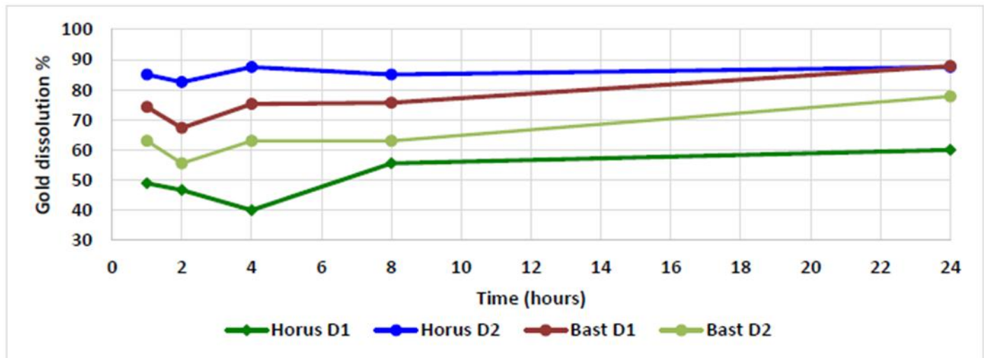
Figure 10.2. Flotation tail cyanidation gold extraction.
