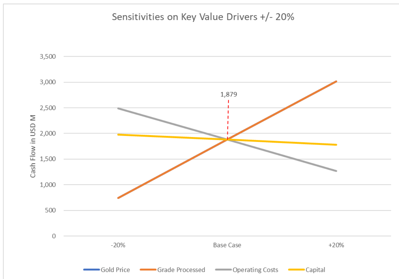
Figure 19.1. Sukari Mineral Reserve (100% basis) sensitivity analysis (±20%) for key value drivers (numbers as after-tax NPV 5 , in $M).
