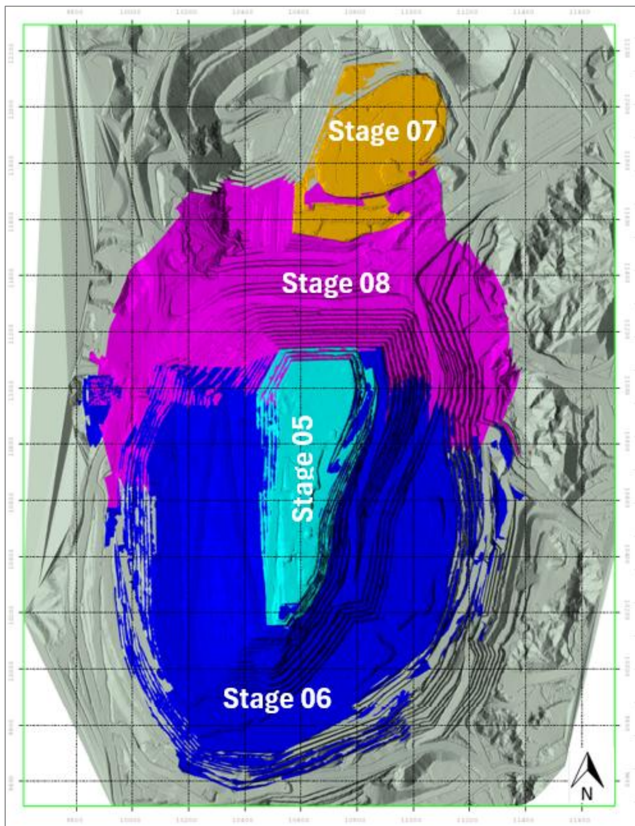
Figure 13.1. Remaining open pit stages at Sukari open pit.
