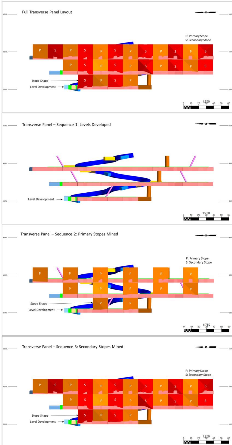
Figure 13.3 Schematic transverse long-hole stoping progression.
