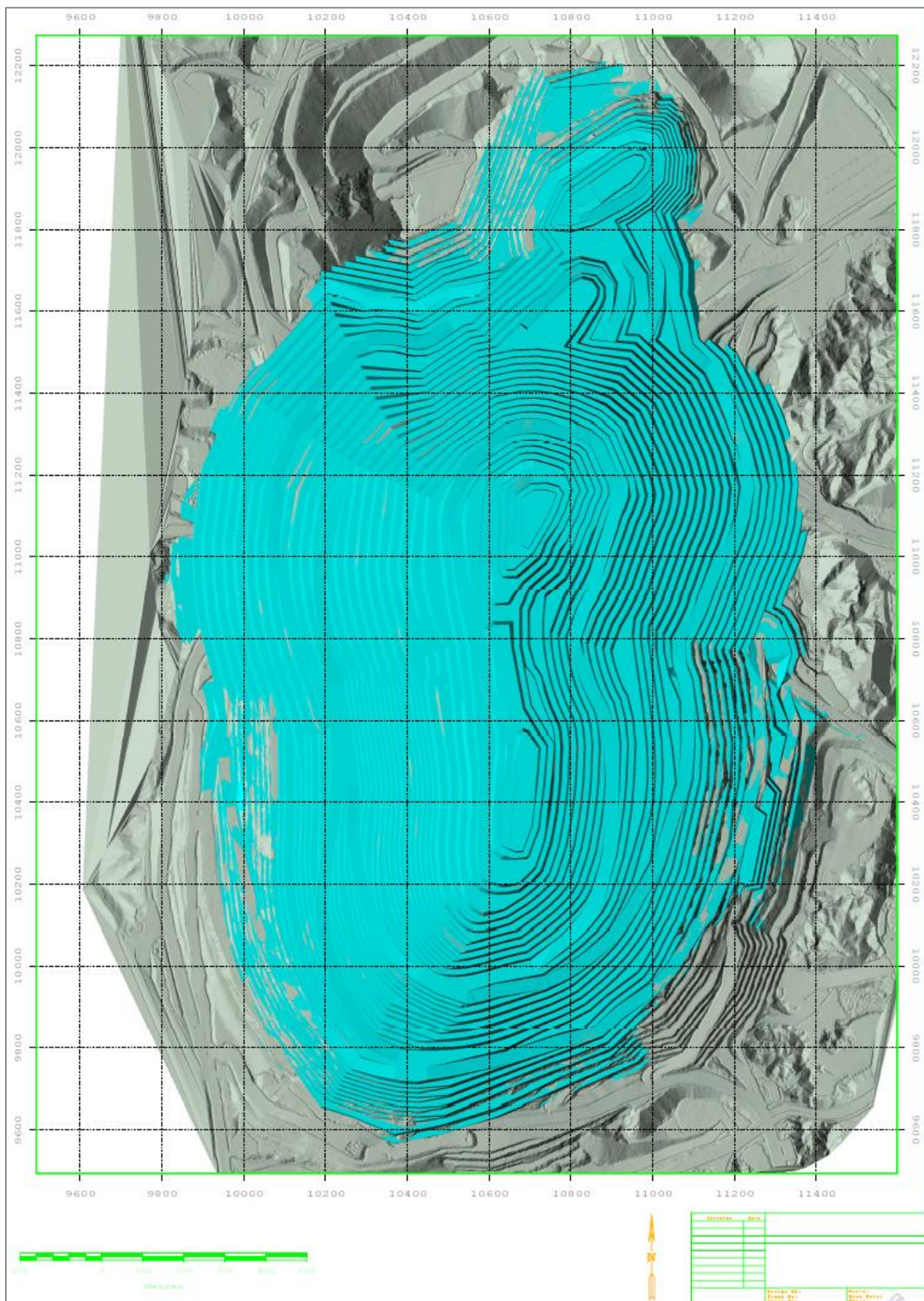
Figure 12.2. LOM design.
