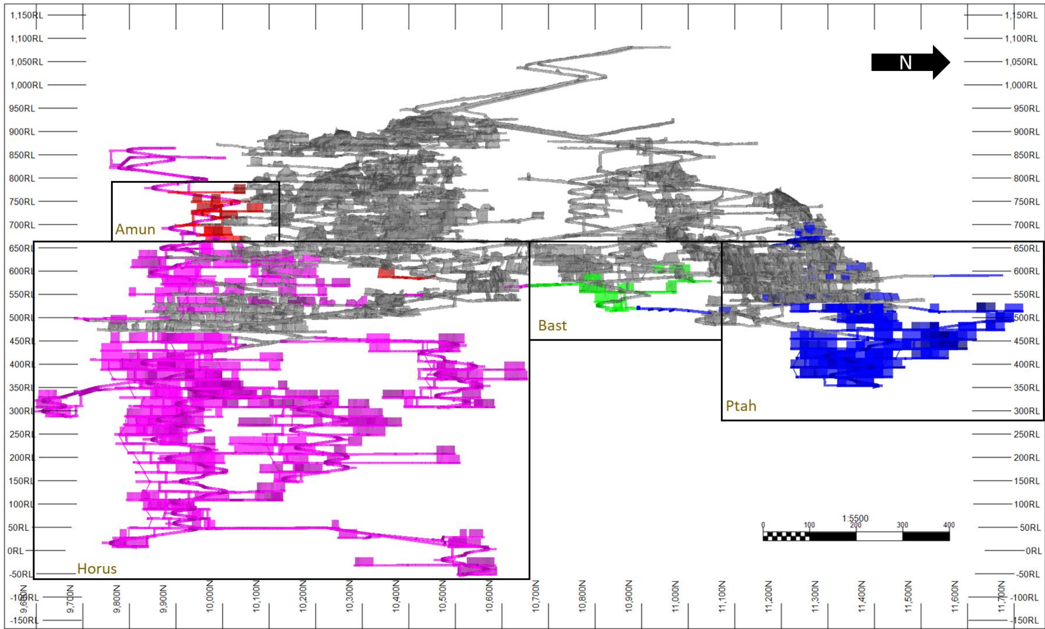
Figure 13.2. Map of the final underground mine outline.
