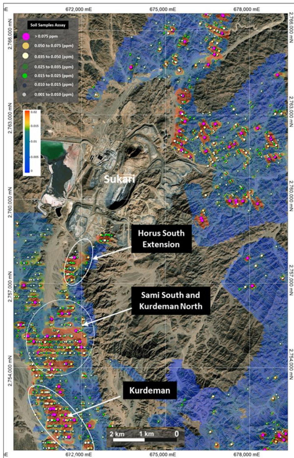
Figure 7.2. Sukari licence, soil sampling results.
