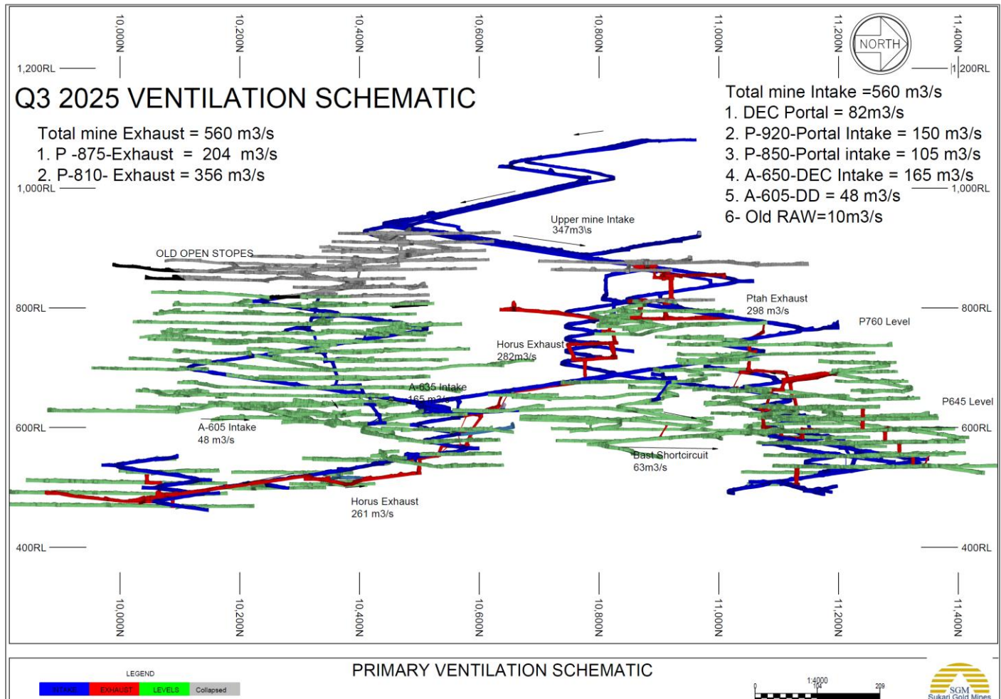
Figure 13.5. Sukari primary ventilation schematic.
