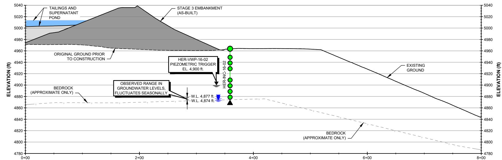
2 SECTION A.1 HER-INC-16-02 FIG SCALE A
