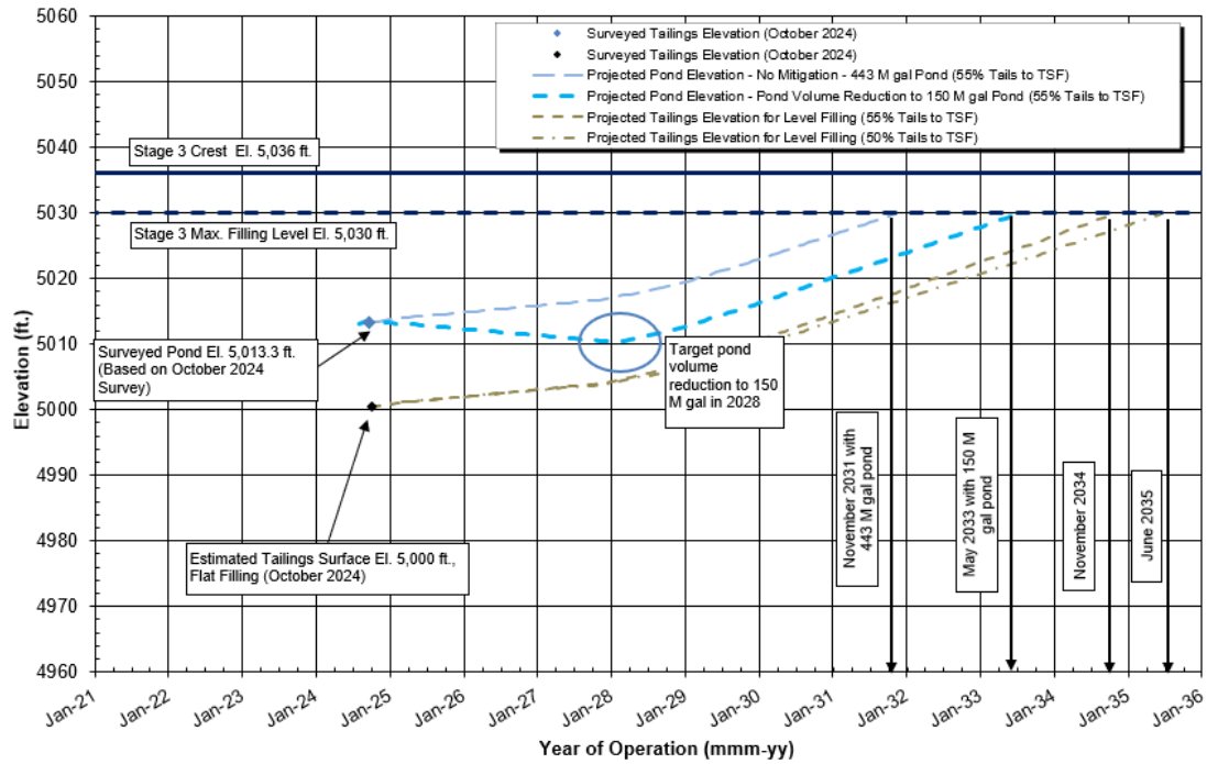
Figure A.3 TSF Filling Curve
