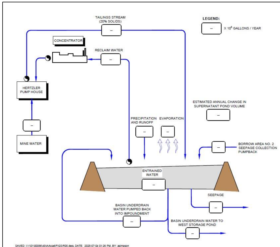
Figure A.4 Water Balance Flowsheet
