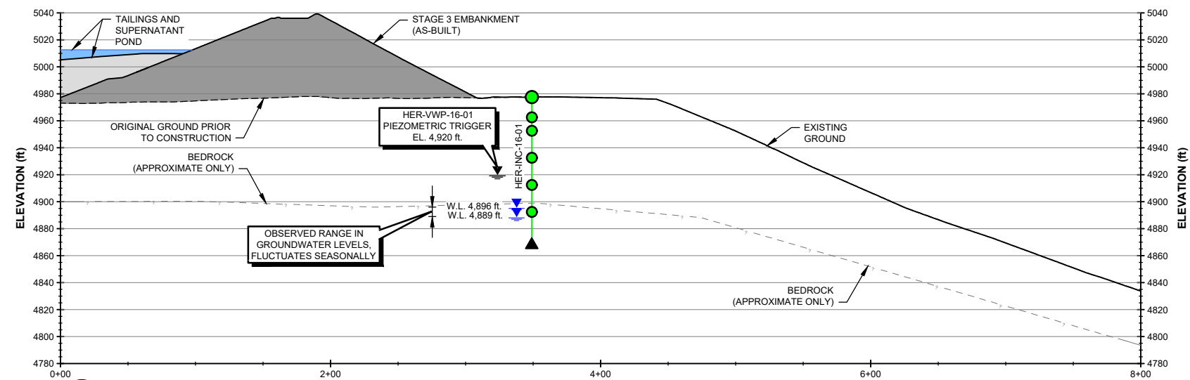
1 SECTION A.1 HER-INC-16-01 FIG SCALE A
